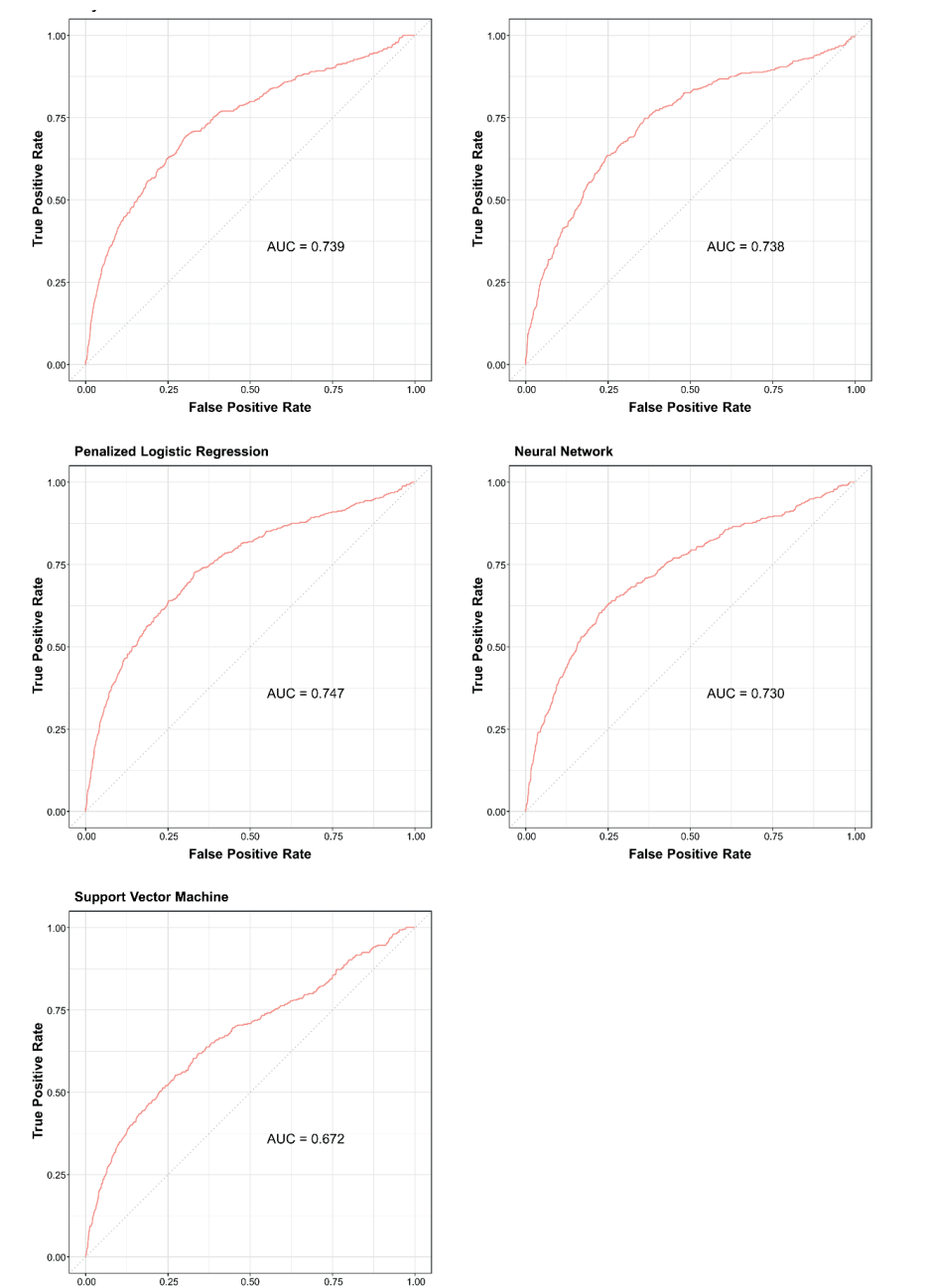
Figure 2. The receiver operating characteristic (ROC) curve and area under the curve (AUC) for each machine learning prediction model in the derivation-cohort.
