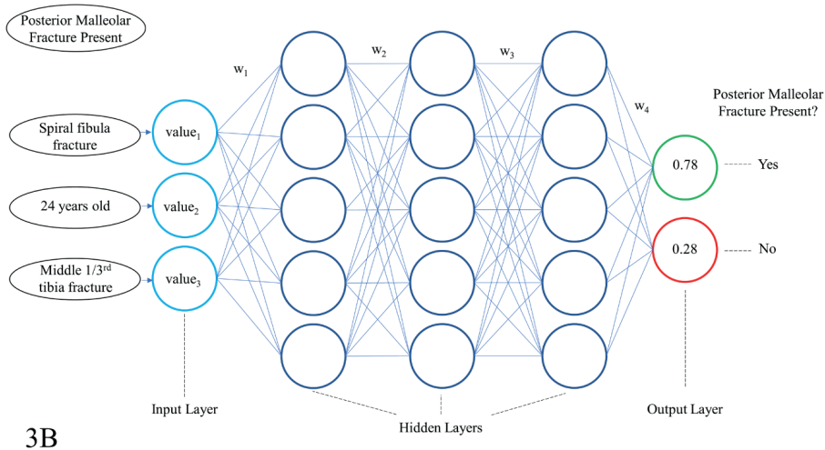
Figure 3 A simplified example of a neural network.
