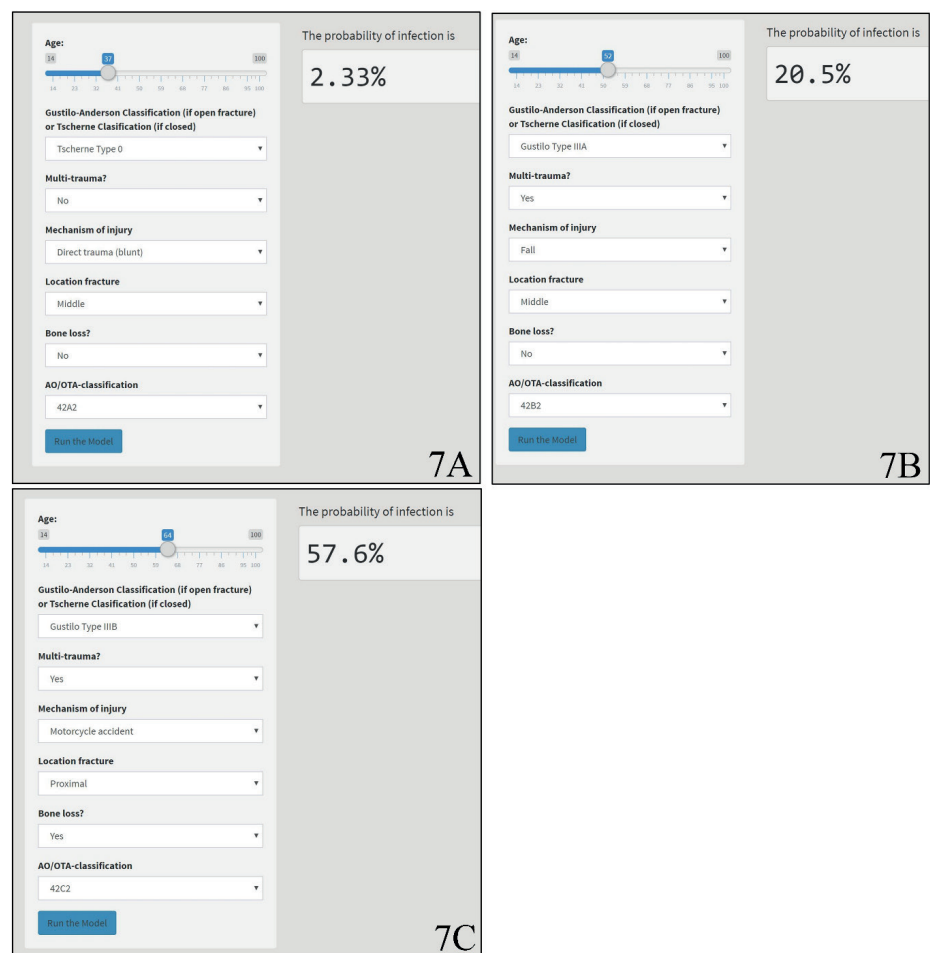
Figure 7. Probabilities generated by the prediction tool for three fictitious case scenarios. 7A. For a 37-year old patient who sustained a blunt trauma resulting in a closed, Tscherne type 0, oblique, middle third tibia shaft fracture without bone-loss, the prediction tool generated a 2.3% probability of infection. 7B. For a 52-year old multi-trauma patient with a complex (AO/OTA type 42B2), open (Gustilo-Anderson type IIIA), middle third tibia shaft fracture after a fall, without bone-loss, the prediction tool generates a 20.5% probability of infection. 7C. For a 64-year old multi-trauma patient with a complex (AO/OTA type 42C), open (Gustilo-Anderson type IIIB), proximal third tibia shaft fracture after a motorcycle accident with bone loss, the prediction tool generates a 57.6% probability.
